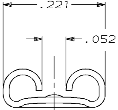
VIEW X-X SCALE 8:1
